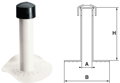
SEMPLICE H 400 MM IN POLIOLEFINE (TPO) SIMPLE H 400 MM MADE OF POLYOLEFYNE (TPO)
