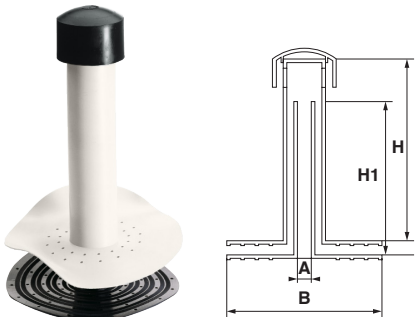
DOPPIO H 400 MM IN POLIOLEFINE (TPO) DOUBLE H 400 MM MADE OF POLYOLEFYNE (TPO)
